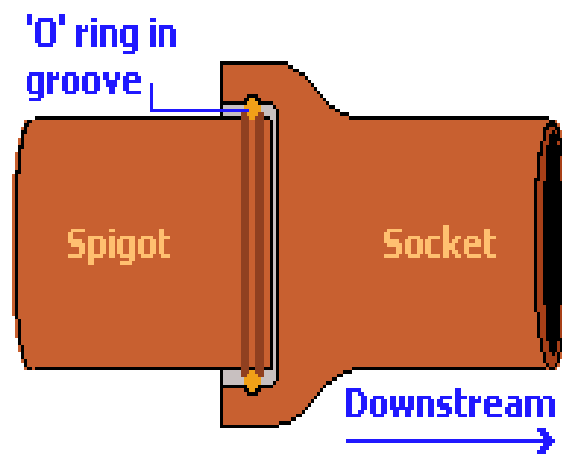
Fig: Spigot and Socket Joint
